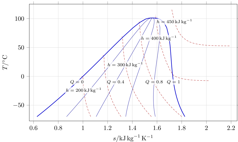
R134a temperature-entropy diagram
