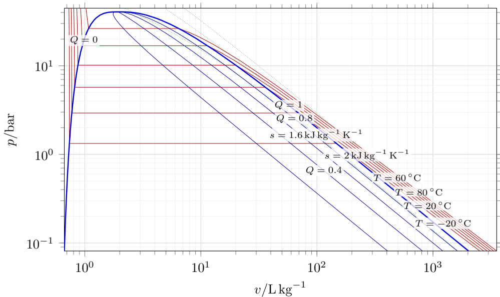
R134a pressure-specific-volume diagram
