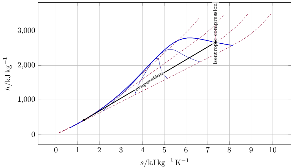
Water HS background and process paths
